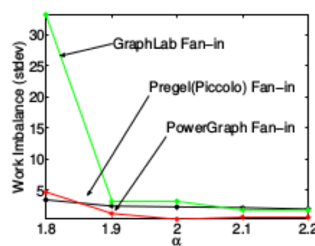
(a) Power-law Fan-In Balance
