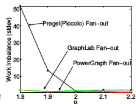
(b) Power-law Fan-Out Balance
