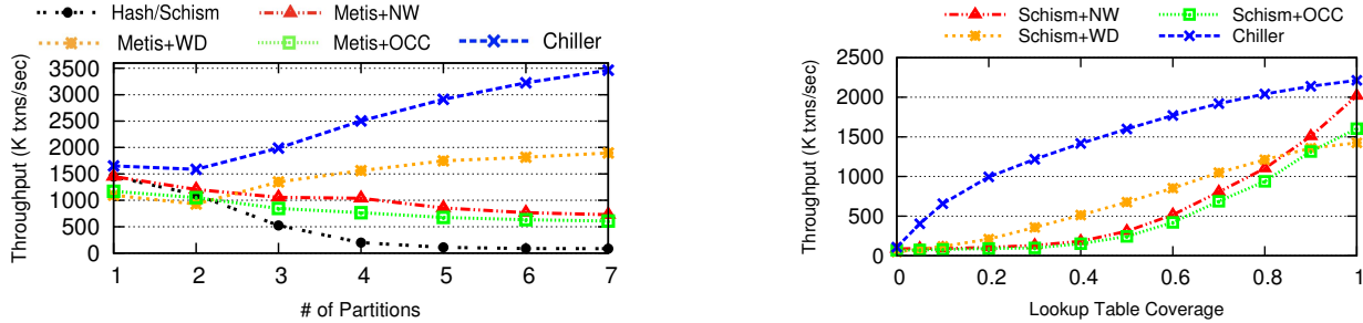
Figure 9: YCSB distributed with increasing cluster sizes.
