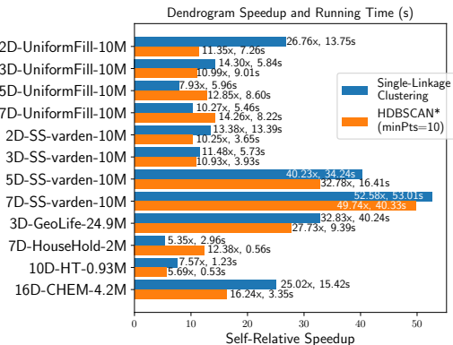
Figure 9: Self-relative speedups and times for ordered dendrogram computation for single-linkage clustering and HDBSCAN* (minPts = 10). The x -axis indicates the self-relative speedup on 48 cores with hyper-threading. The speedup and time is shown at the end of each bar.
