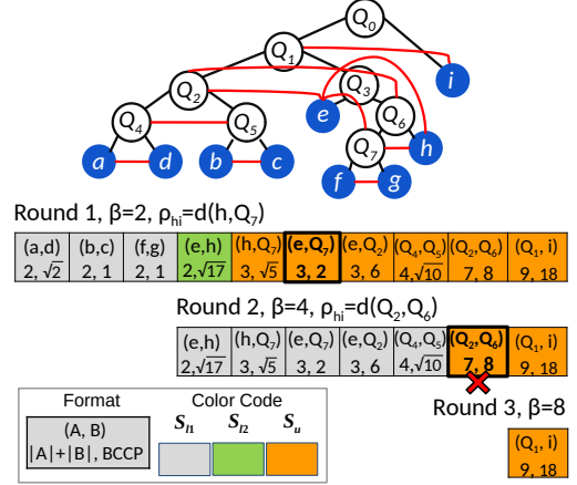
Figure 2: This is an example for both GFK (Algorithm 2) and MEMoGFK (Algorithm 3) for EMST corresponding to the data set shown in Figure 1. The red lines linking tree nodes and the boxes drawn below represent well-separated pairs. The boxes also show the cardinality and BCCP value of the pair. Their correspondence with the symbols S_{11}, S_{12} , and S_u from the pseudocode are color-coded. The pairs that generate \rho_{hi} are in bold squares, and the pairs filtered out have a red cross. Using our MemoGFK optimization, only the pairs in S_{11} needs to be materialized, in contrast to needing to materialize all of the pairs in GFK.
